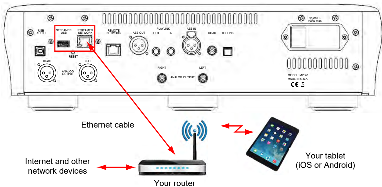
Stream-X2 connections on back panel of MPS-8
